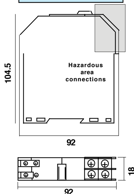
Housing Dimensions
