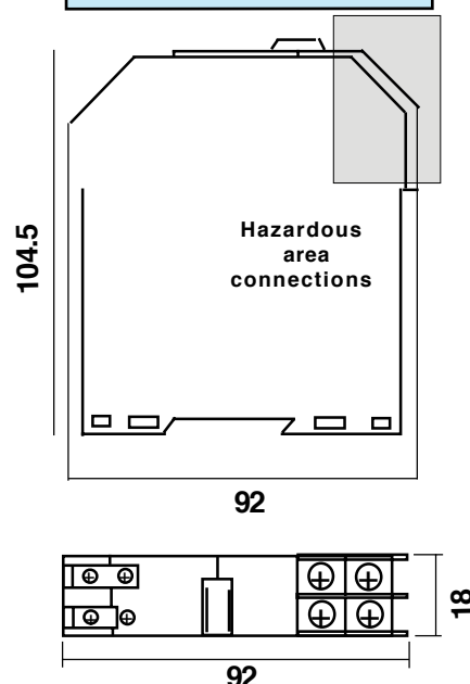
Housing Dimensions
