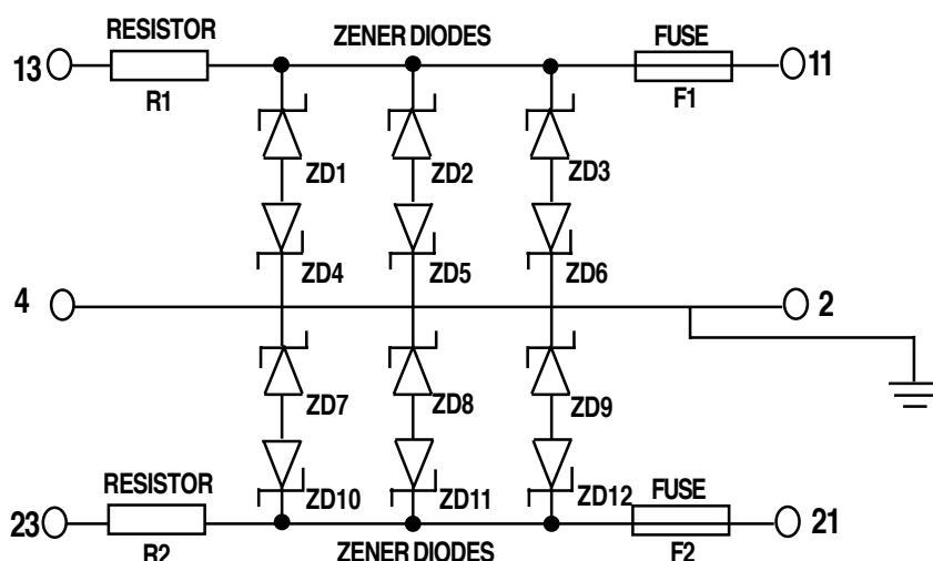
Connection Diagram
