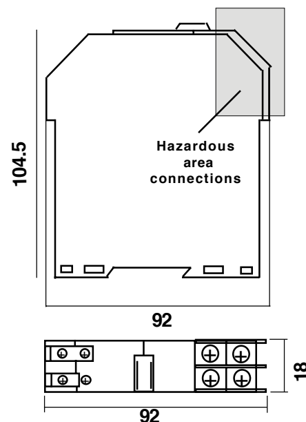
Housing Dimensions
