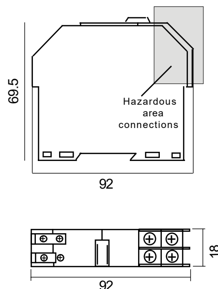
Housing Dimensions
