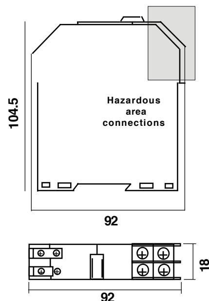
Housing Dimensions
