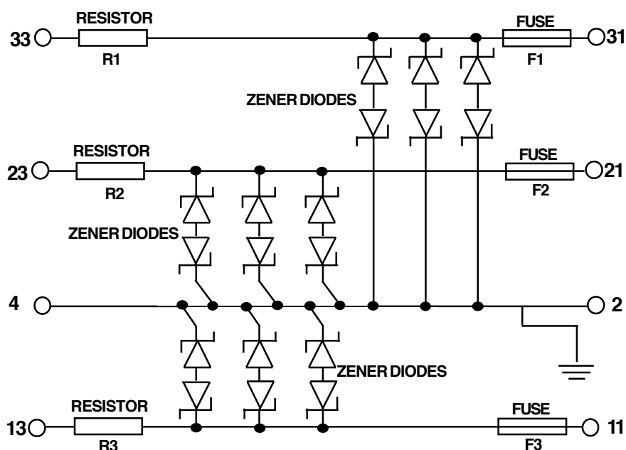
Connection Diagram
