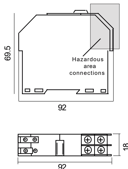
Housing Dimensions
