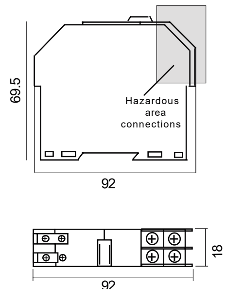
Housing Dimensions
