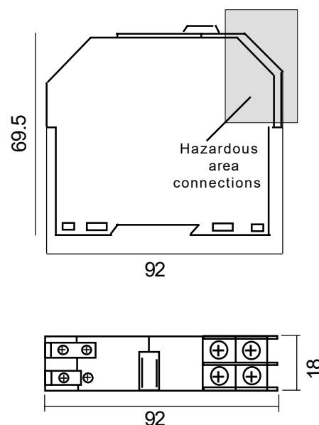
Housing Dimensions
